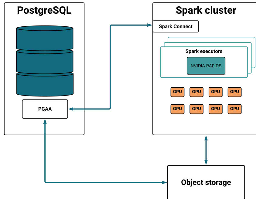
図 1: Spark Rapid Architecture
