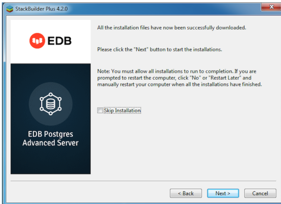
Fig. 2: Installing Slony
