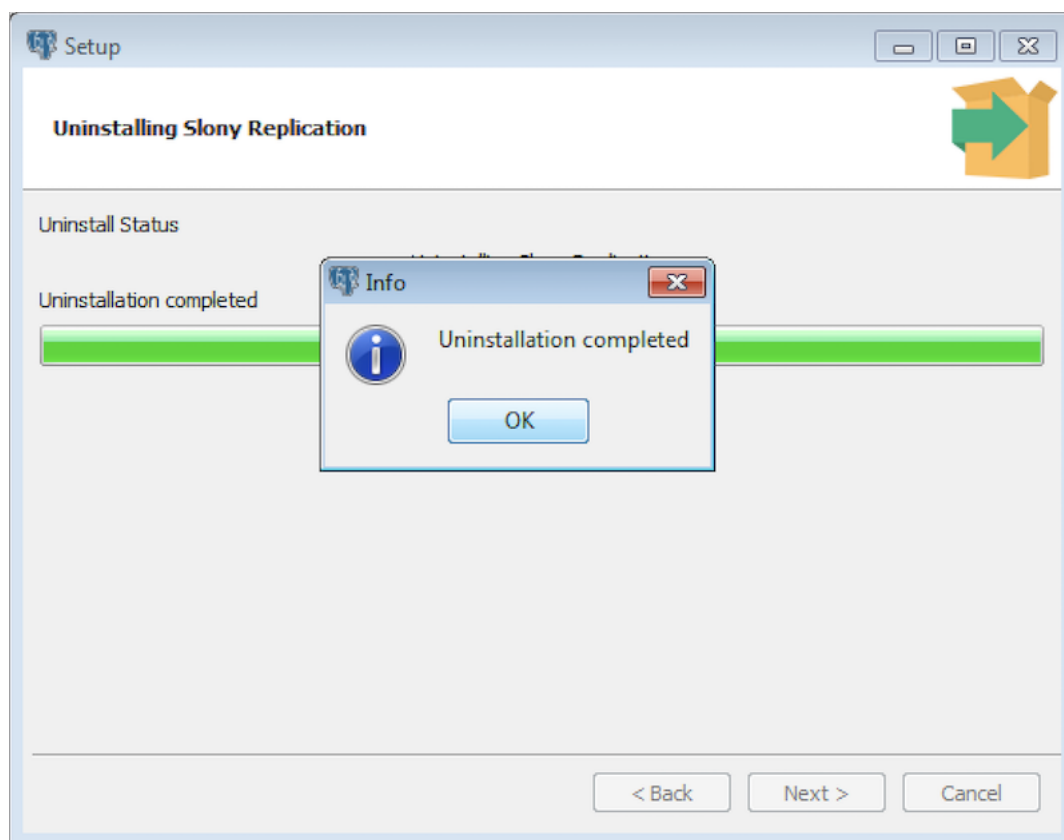
Fig. 2: Uninstallation completes
