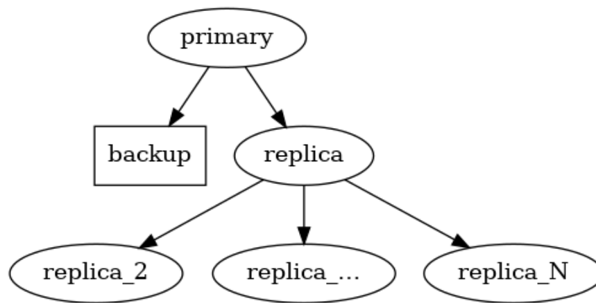
Fig. 1: Cluster with cascading replication
